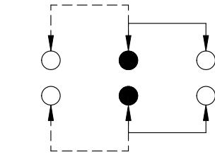
SCHEMATIC (NON-SHORTING)
